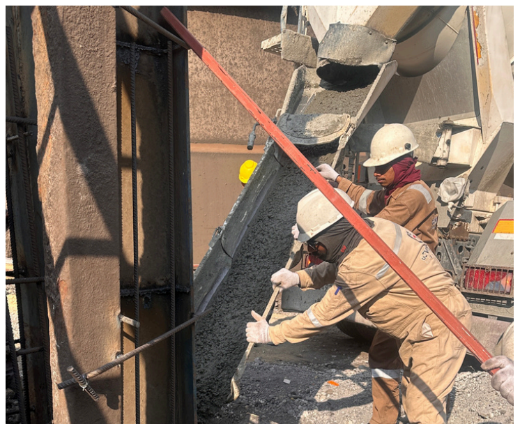
COLUMN STRENGTHENING
